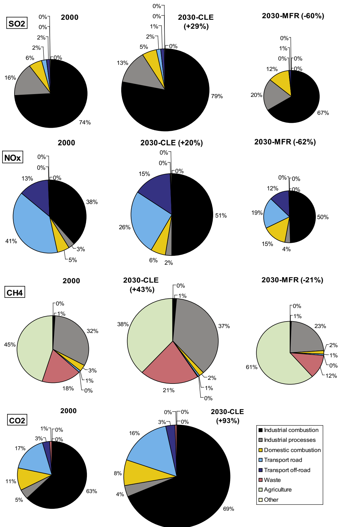
Fig. 8. Source sector contribution to the global emissions of selected aerosols and greenhouse gases; Source: GAINS model.
