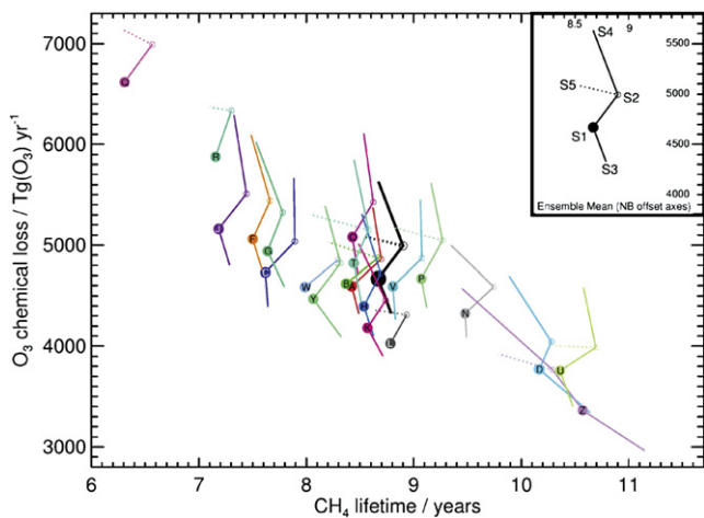
Fig. 20. Response of global CH 4 lifetime to various scenarios across 21 models (S1 = 2000; S2 = 2030 B2 + CLE; S3 = 2030 B2 + MFR; S4 = 2030 A2; S5 = 2030 B2 + CLE + climate change) (From Stevenson et al. (2006)).
