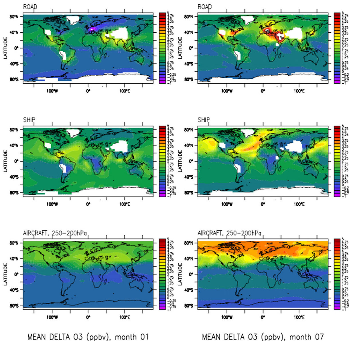
Fig. 35. Mean perturbations of ozone (ppbv) in the PBL (surface–800 hPa) for road emissions (upper row), ship emissions (middle row), and in the upper troposphere (200–250 hPa) for aircraft emissions (lower row) during January (left column) and July (right column) (Hoor et al., 2009).
