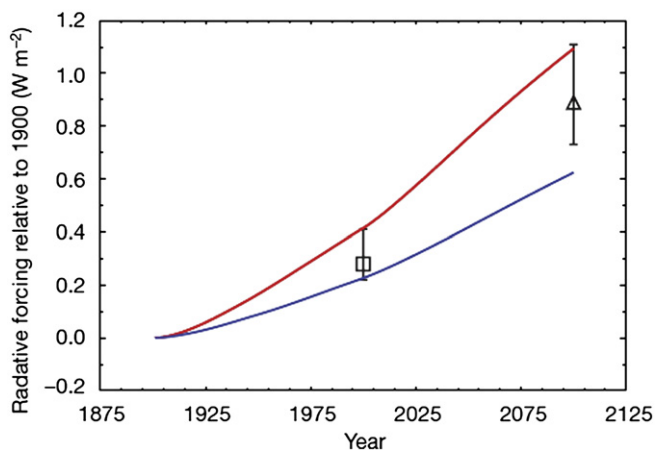
Fig. 27. Indirect radiative forcing due to ozone on plants affecting the \text{CO}_2 uptake for 'high' (red) and 'low' (blue) plant sensitivity to ozone (from Sitch et al. (2007)). Direct radiative forcing due to ozone is included as bars.
