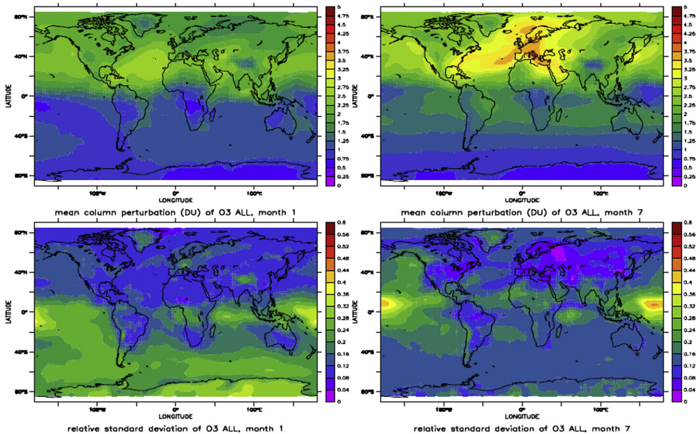
Fig. 32. Top panels: Mean column ozone perturbations due to all types of transport, as simulated by the TM4, LMDzINCA, OsloCTM2 and p-TOMCAT models (ensemble mean) for January (left) and July (right). Bottom panels: Corresponding relative standard deviations for January (left) and July (right) (from Hoor et al., 2009).
