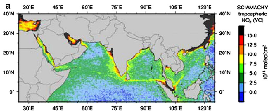
Fig. 33. NO x signature of shipping in the Indian Ocean as observed by satellite (from Richter et al., 2004).
