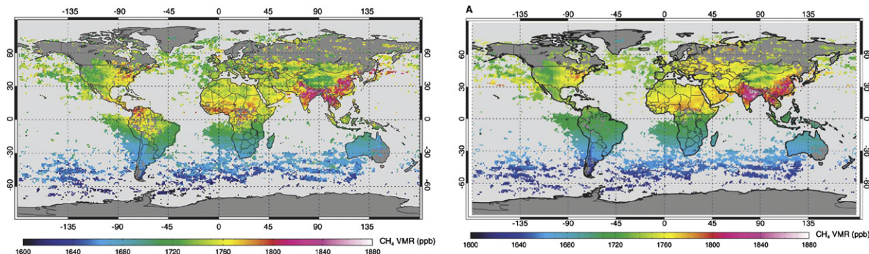
Fig. 10. SCIAMACHY measurements of column-averaged methane mixing ratios in ppb (left) and TM3 model results of column averaged CH 4 mixing ratios (right), averaged for the time period August -November 2003 (Frankenberg et al. (2005)).
