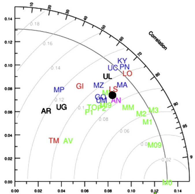
Fig. 21. Taylor plot exhibiting AOD standard deviation (x & y axis) and correlation (angular component), showing year 2000 performance of 16 AeroCom A models (blue and red symbols: higher and lower resolution CTM's or nudged GCMs, black symbols: not nudged GCMs) against 12 months (April 2000–March 2001) of MODIS satellite derived aerosol optical depth at 550 nm. Shown is also the performance of other satellite data sets (green symbols: Polder 1 and 2, AVHRR, TOMS MISR and Modis from other years). The black ball represents the behaviour of the AeroCom median model constructed from the 16 AeroCom A model results. Data correspond to model results documented in Textor et al. (2006) and Kinne et al. (2006).
