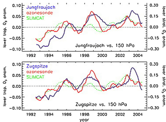
Fig. 42. 12-month running means of the normalized monthly anomalies with respect to the 1992–2004 mean annual cycle of lower free tropospheric ozone (blue) at (top) Jungfraujoch and (bottom) Zugspitze, and 150 hPa (~13.6 km altitude) ozone averaged for Payerne and Hohenpeissenberg (red). From Ordóñez et al., 2007.
