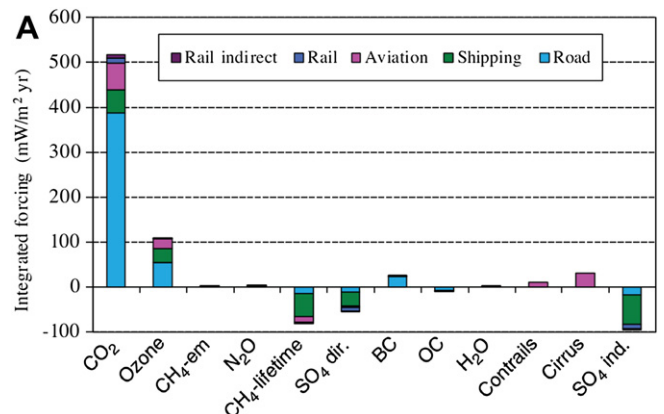
Fig. 38. Integrated radiative forcing of current emissions, by substance and transport subsector, over different time horizons. (A) Integrated global mean RF (mW m 2 yr) due to 2000 transport emissions, time horizon H = 100 years. (From Fuglestedt et al., 2008)
