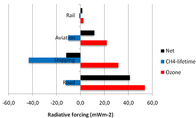
Fig. 37. Radiative forcing due to ozone, impact of changes in CH 4 lifetime, and the corresponding net radiative forcing for four transport sectors from pre-industrial to present, as calculated by Fuglestedt et al. (2008).
