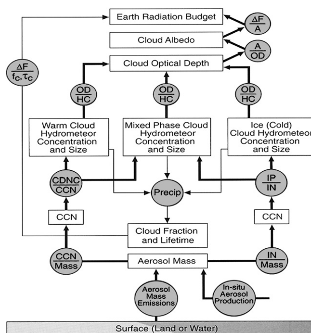
Fig. 3. Flow chart showing the processes linking aerosol emissions/production, cloud condensation nuclei (CCN), cloud droplet number concentration (CDNC), ice nuclei (IN), ice particles (IP), optical depth (OD), hydrometeor (HC), albedo (A), cloud fraction ( f_c ), cloud optical depth ( \tau_c ) and radiative forcing ( \Delta F ) (Adopted from IPCC, 2001).
