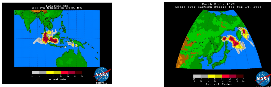
Fig. 7. a-b. The aerosol index as derived from TOMS observations.
